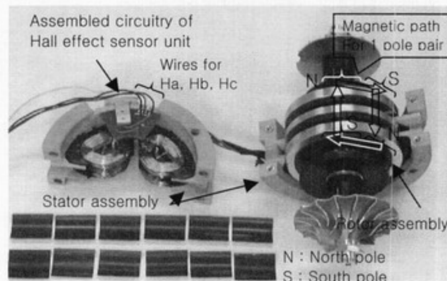
Fig. 1 Photograph of the overall structure of a fan cake Brushless DC Motor with axial air gap
